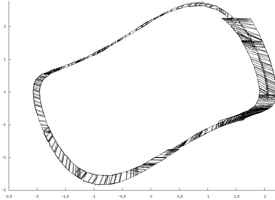
Fig. 2. Reachable sets for the van der Pol system during time intervals
