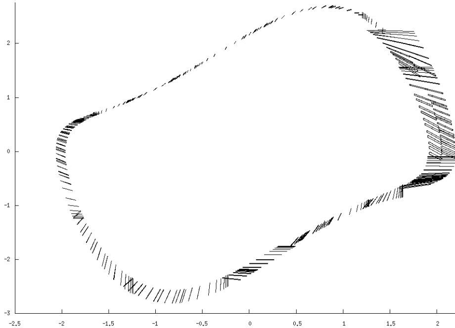
Fig. 1. Reachable sets for the van der Pol system at discretization points
